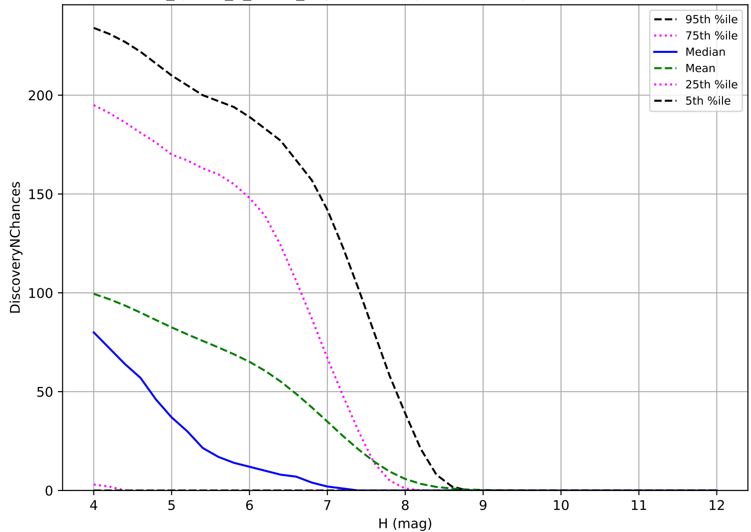
too_ignore_5_4v3.4_10yrs: TNO 3 pairs in 15 nights detection loss
