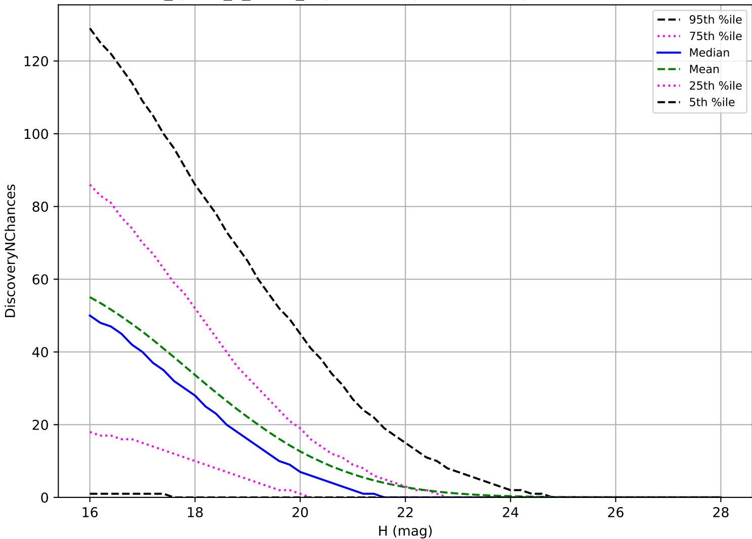
too_ignore_5_4v3.4_10yrs: PHA 3 pairs in 15 nights detection loss
