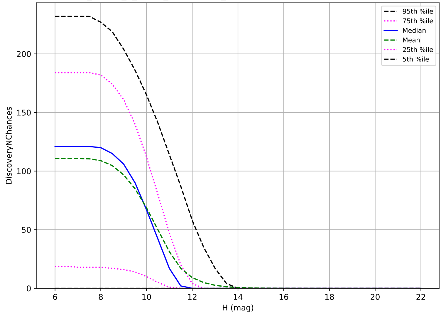
too_ignore_5_4v3.4_10yrs: OCC_r20 3 pairs in 15 nights detection loss
