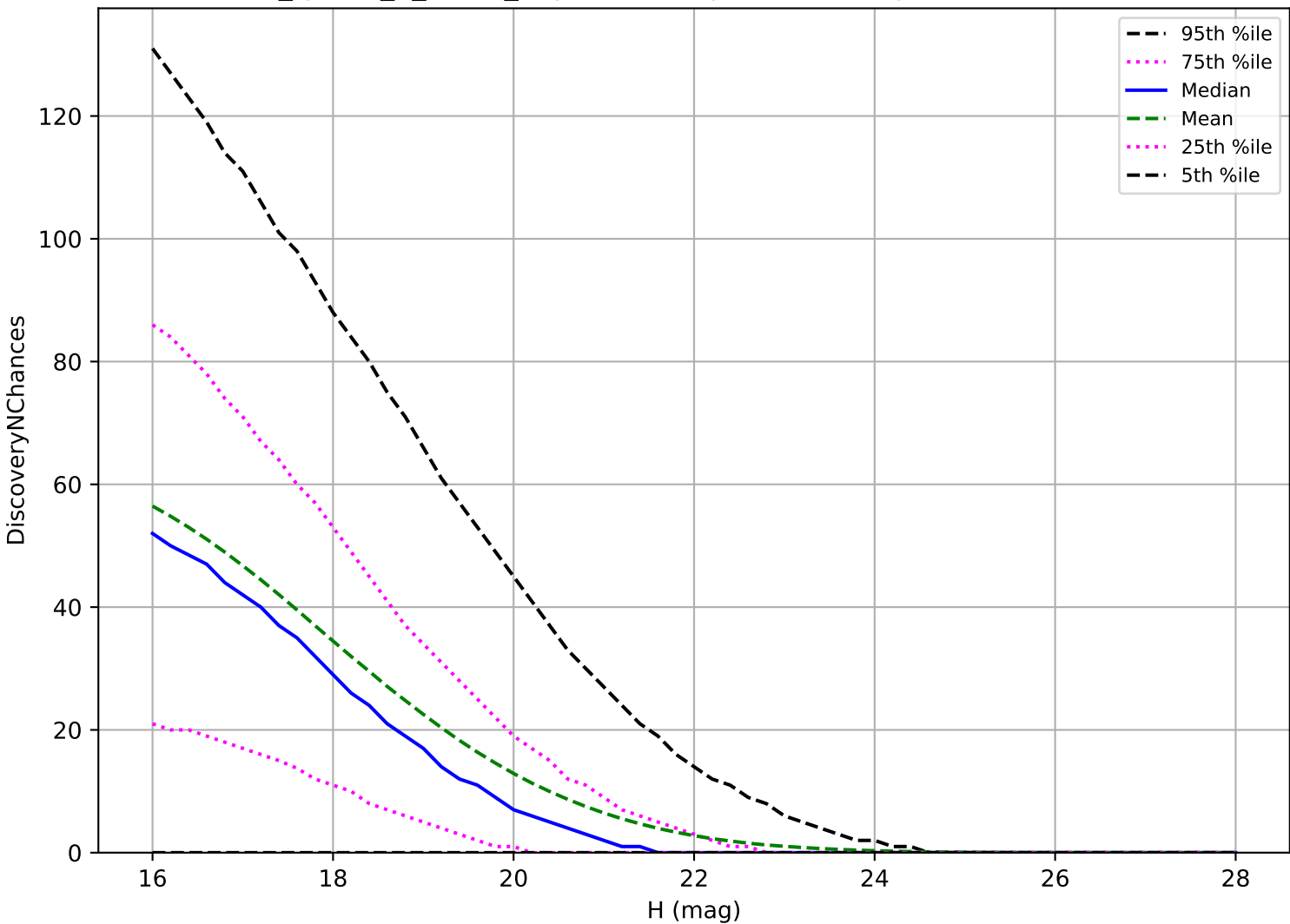
too_ignore_5_4v3.4_10yrs: NEO 3 pairs in 15 nights detection loss
