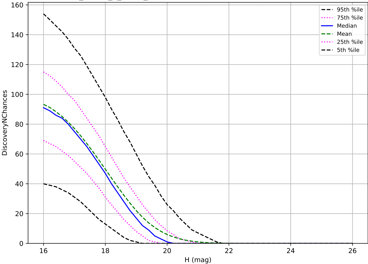
too_ignore_5_4v3.4_10yrs: MBA 3 pairs in 15 nights detection loss
