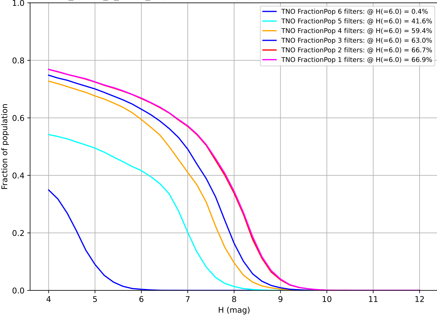
too_ignore_5_4v3.4_10yrs: Fraction of population with colors in X filters TNO
