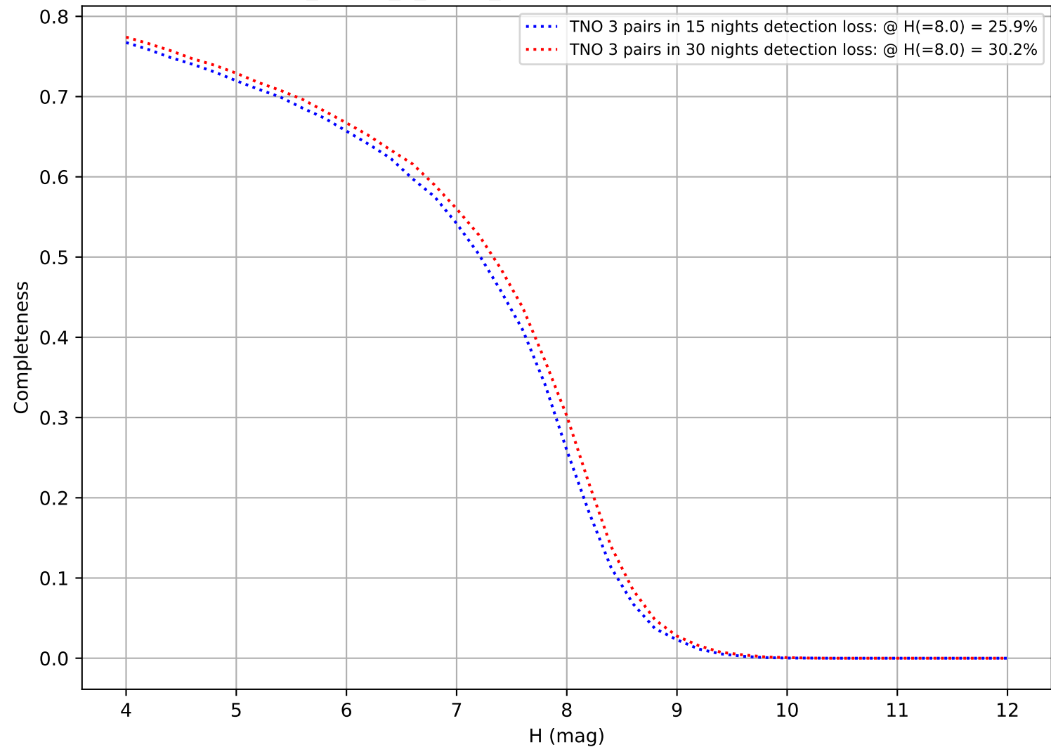
too_ignore_5_4v3.4_10yrs: DifferentialCompleteness
