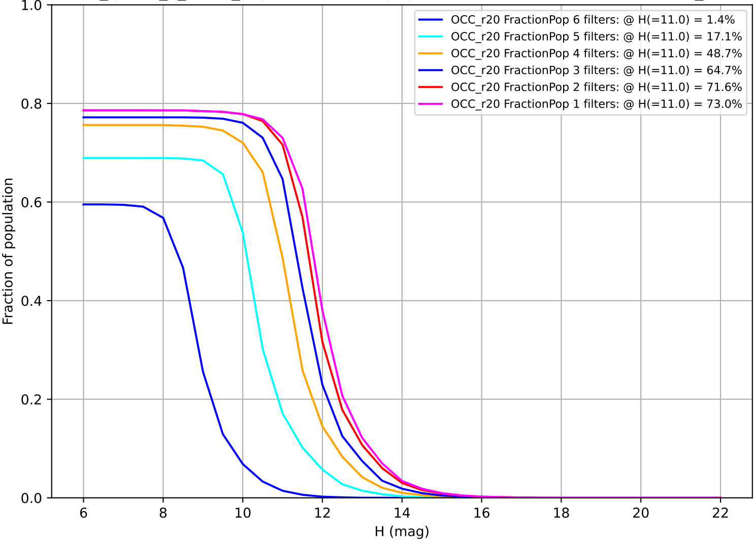
too_ignore_5_4v3.4_10yrs: Fraction of population with colors in X filters OCC_r20
