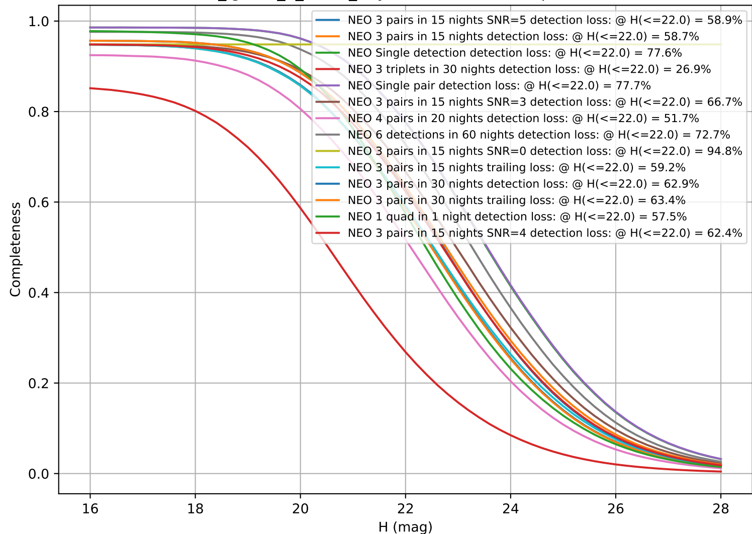
too_ignore_5_4v3.4_10yrs: CumulativeCompleteness
