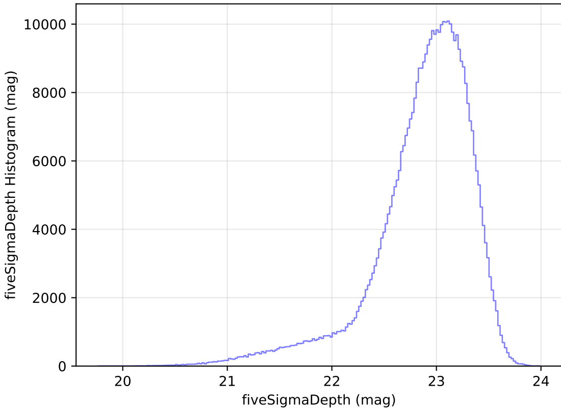
too_ignore_5_4v3.4_10yrs z: fiveSigmaDepth Histogram
