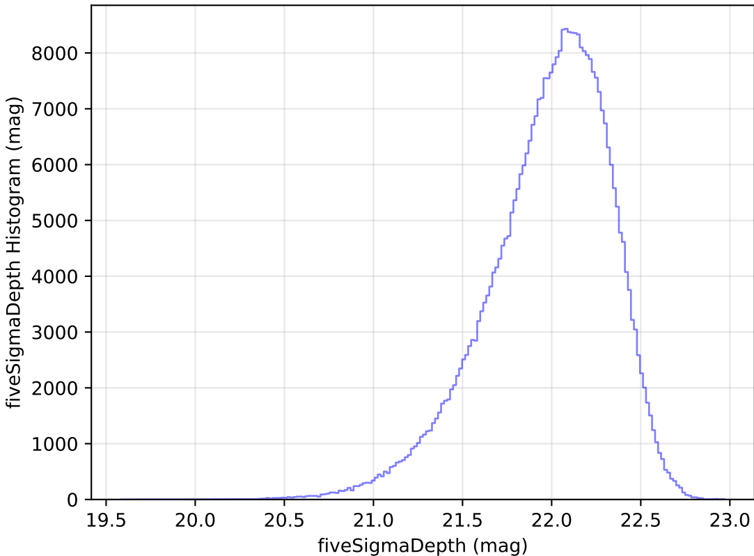
too_ignore_5_4v3.4_10yrs y: fiveSigmaDepth Histogram
