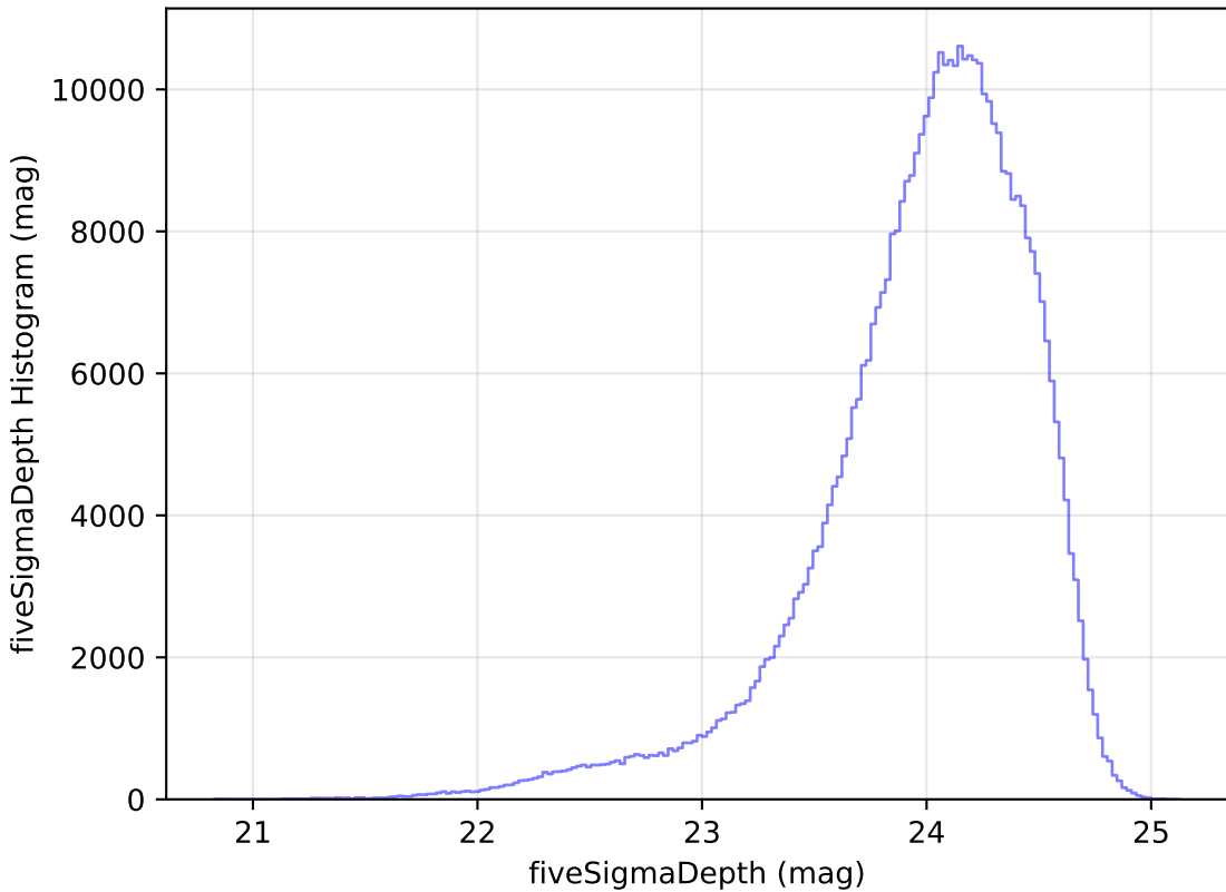
too_ignore_5_4v3.4_10yrs r: fiveSigmaDepth Histogram
