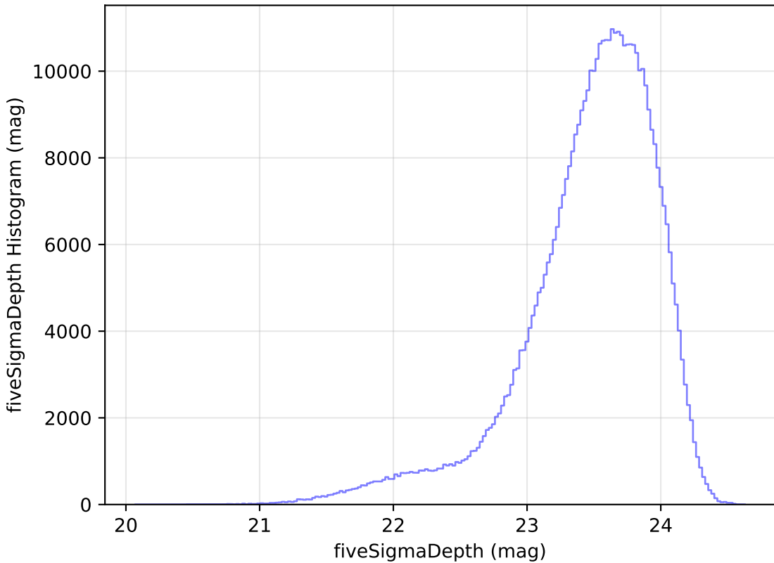
too_ignore_5_4v3.4_10yrs i: fiveSigmaDepth Histogram
