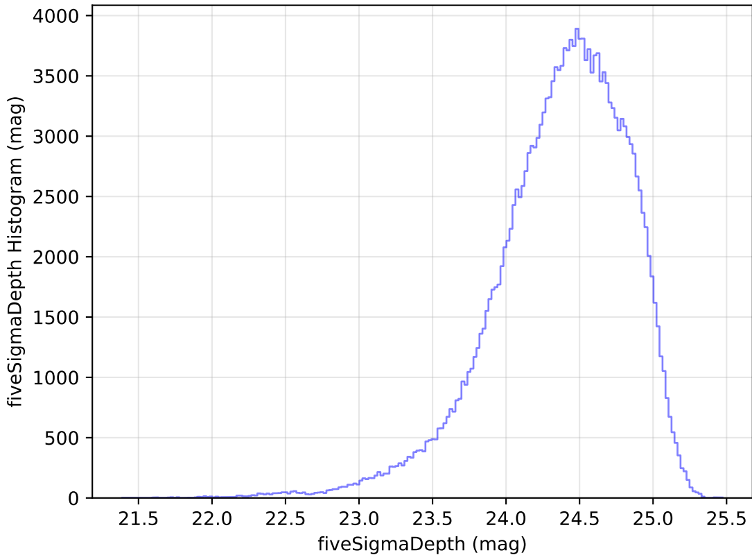
too_ignore_5_4v3.4_10yrs g: fiveSigmaDepth Histogram
