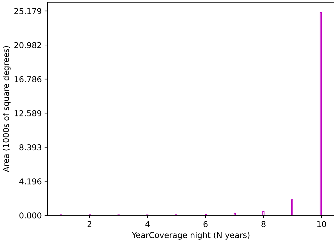
too_ignore_5_4v3.4_10yrs z band: YearCoverage night
