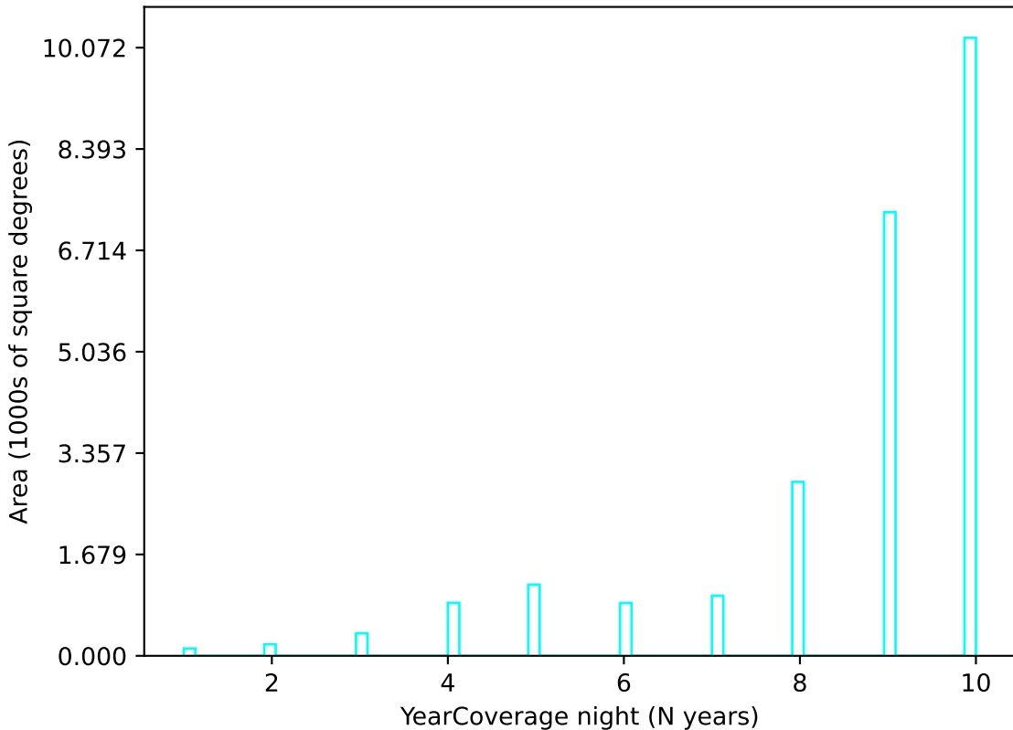
too_ignore_5_4v3.4_10yrs u band: YearCoverage night
