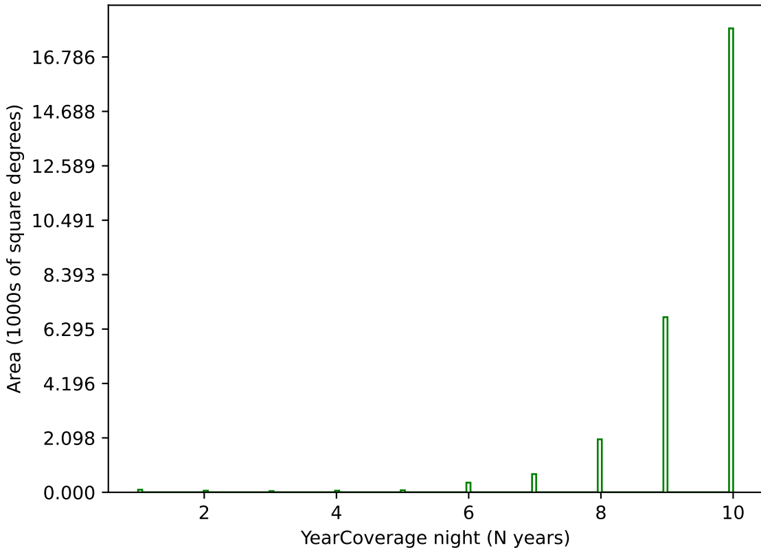
too_ignore_5_4v3.4_10yrs g band: YearCoverage night
