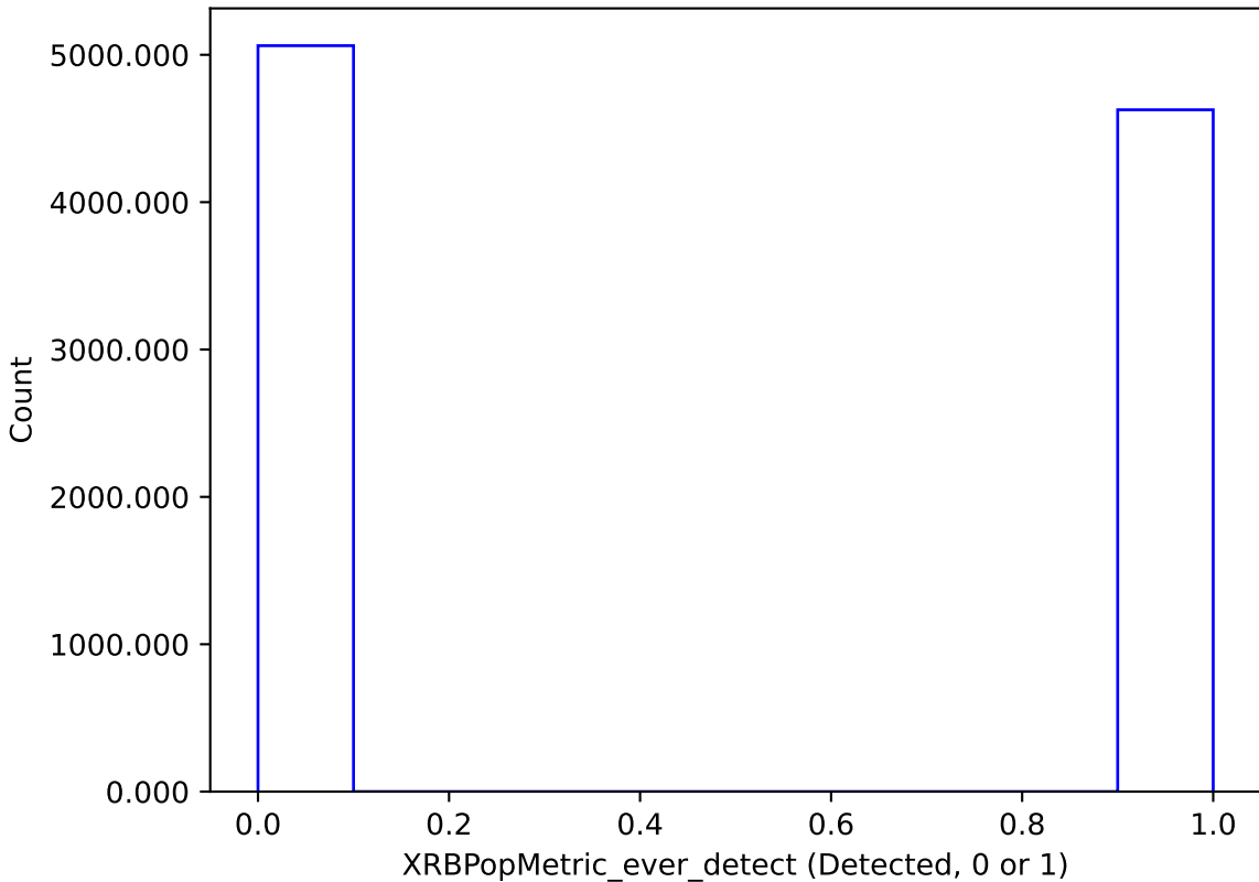
too_ignore_5_4v3.4_10yrs : XRBPoMetric_ever_detect
