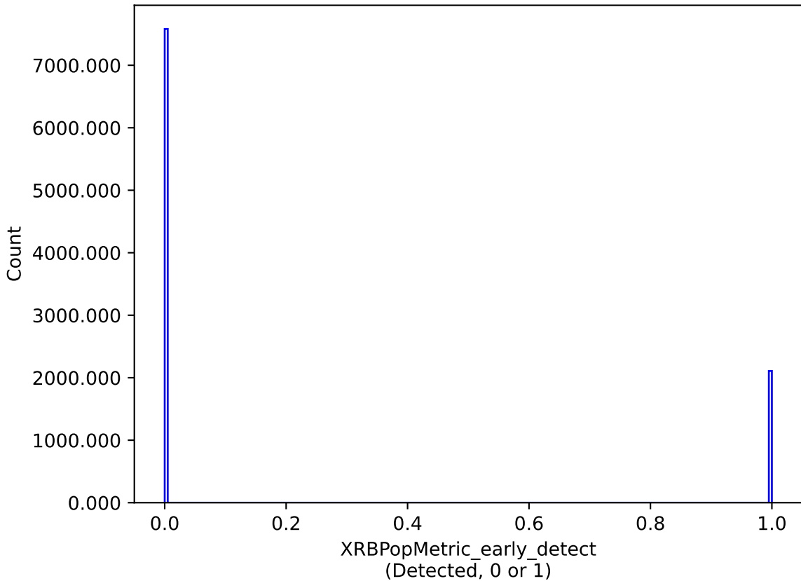
too_ignore_5_4v3.4_10yrs : XRBPoMetric_early_detect
