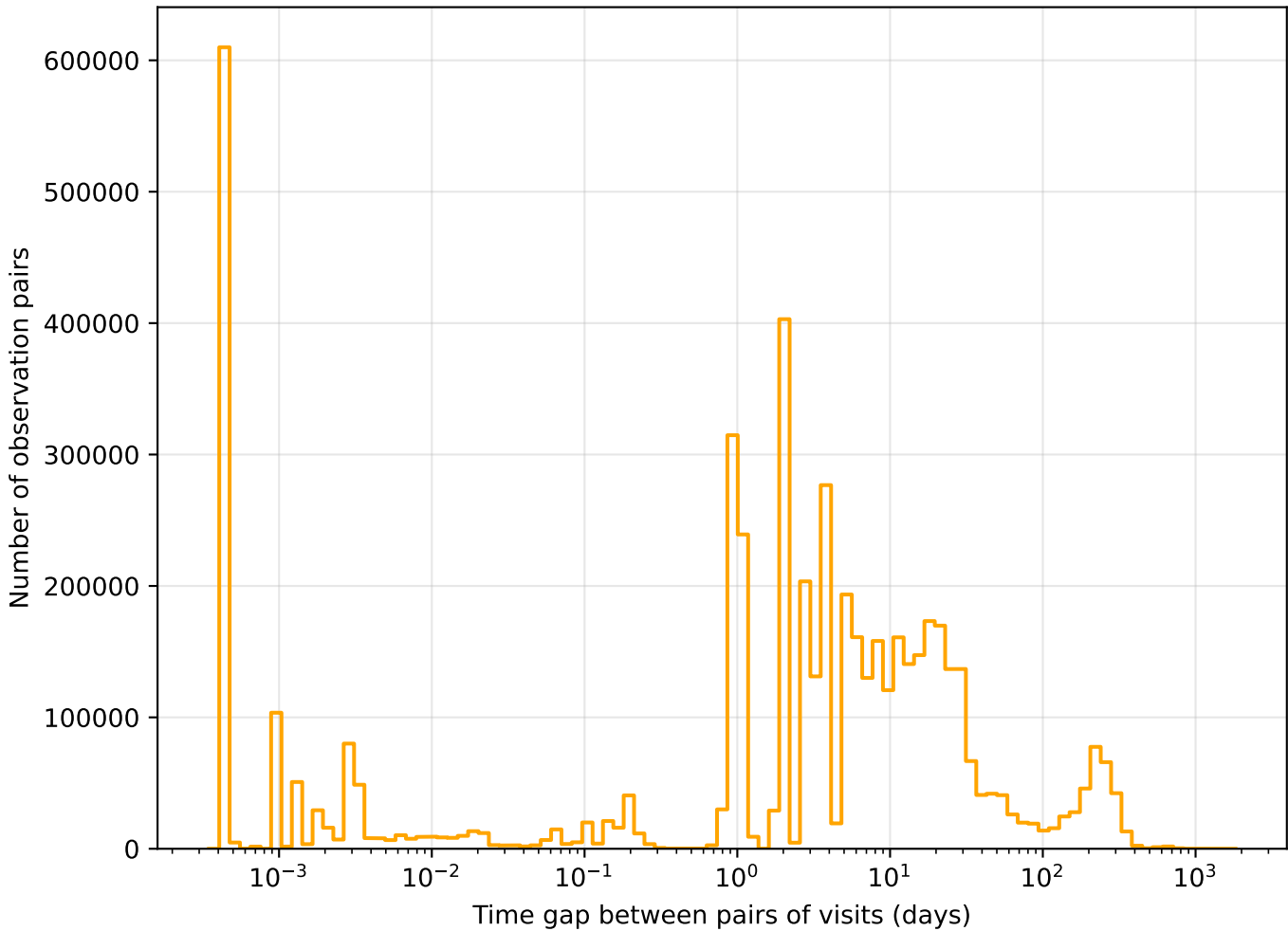
too_ignore_5_4v3.4_10yrs r band: Tgaps observationStartMJD
