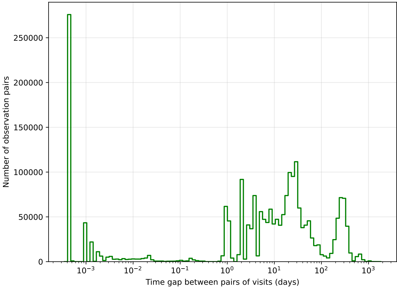
too_ignore_5_4v3.4_10yrs g band: Tgaps observationStartMJD
