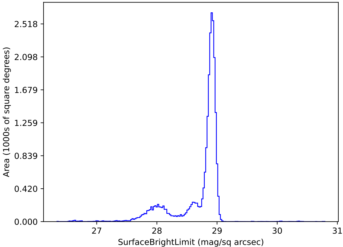
too_ignore_5_4v3.4_10yrs u: SurfaceBrightLimit
