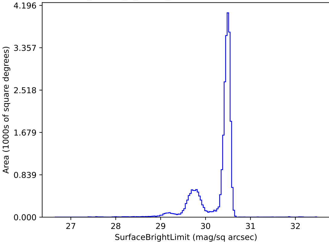
too_ignore_5_4v3.4_10yrs r: SurfaceBrightLimit
