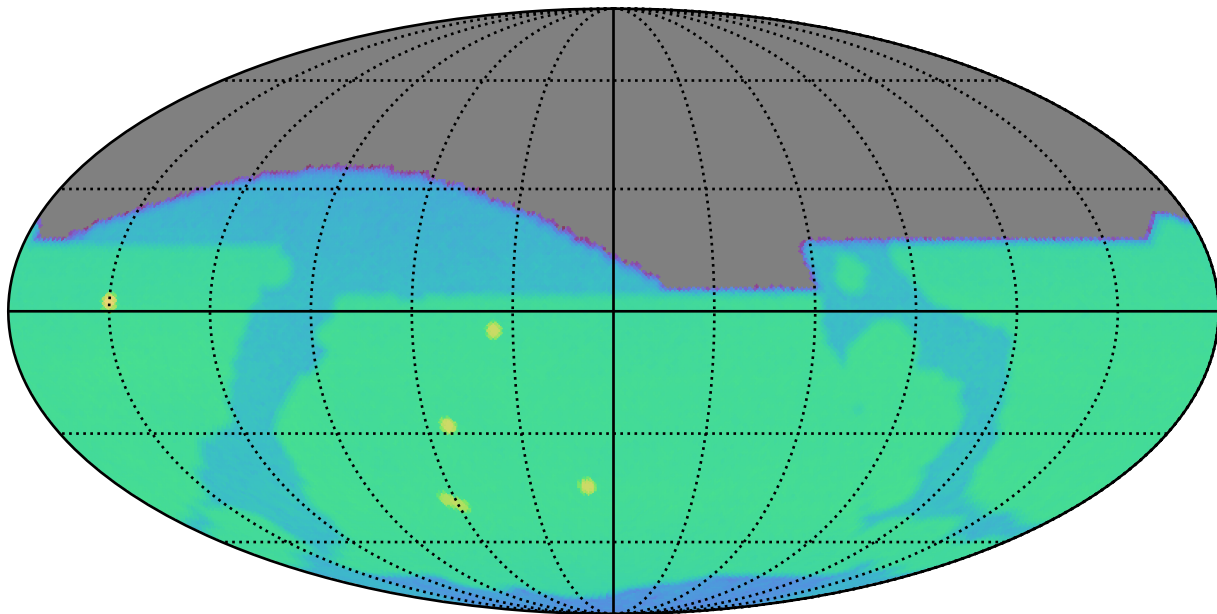
too_ignore_5_4v3.4_10yrs i: SurfaceBrightLimit
