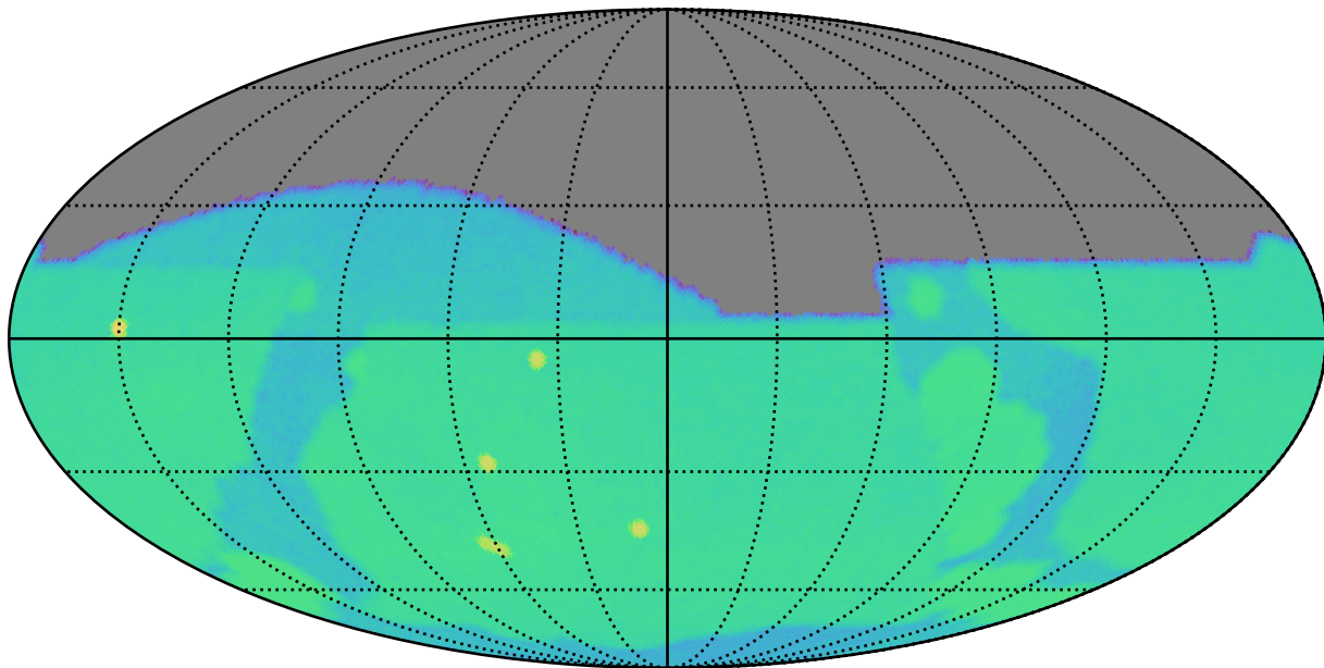
too_ignore_5_4v3.4_10yrs g: SurfaceBrightLimit
