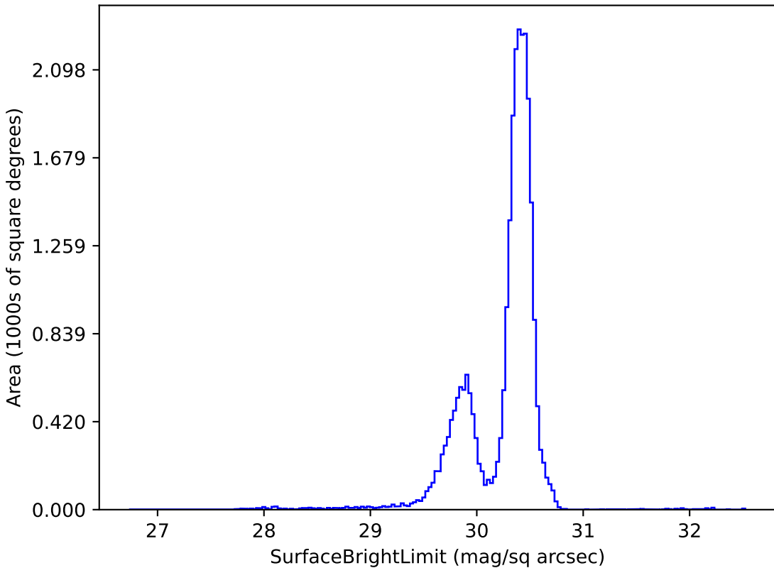
too_ignore_5_4v3.4_10yrs g: SurfaceBrightLimit
