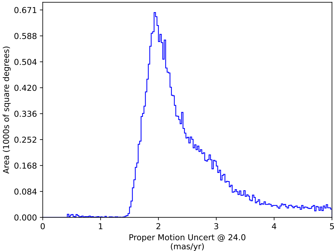
too_ignore_5_4v3.4_10yrs : Proper Motion Uncert @ 24.0
