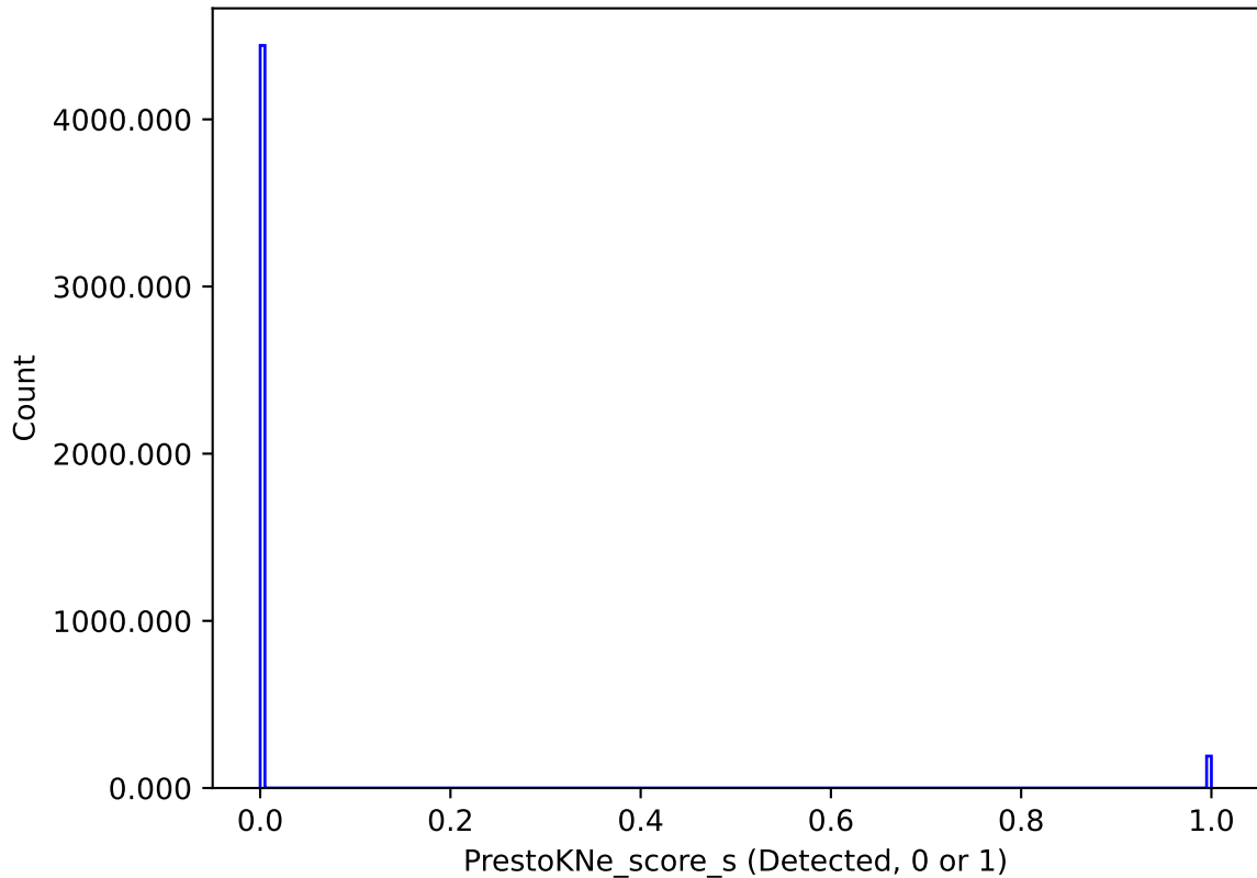
too_ignore_5_4v3.4_10yrs : PrestoKNe_score_s
