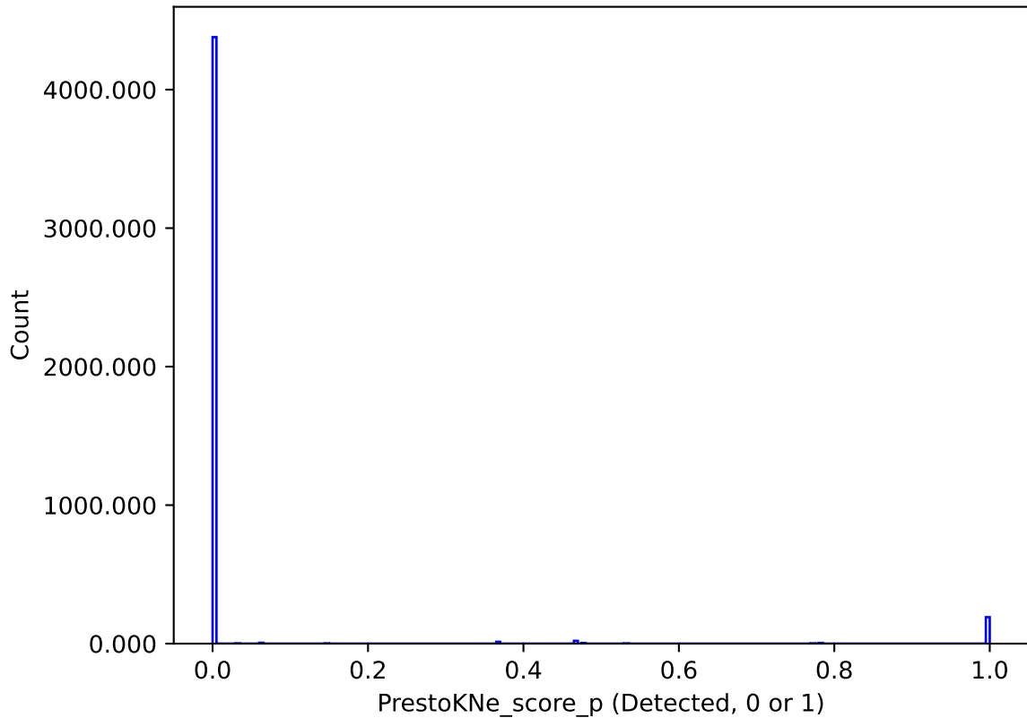
too_ignore_5_4v3.4_10yrs : PrestoKNe_score_p
