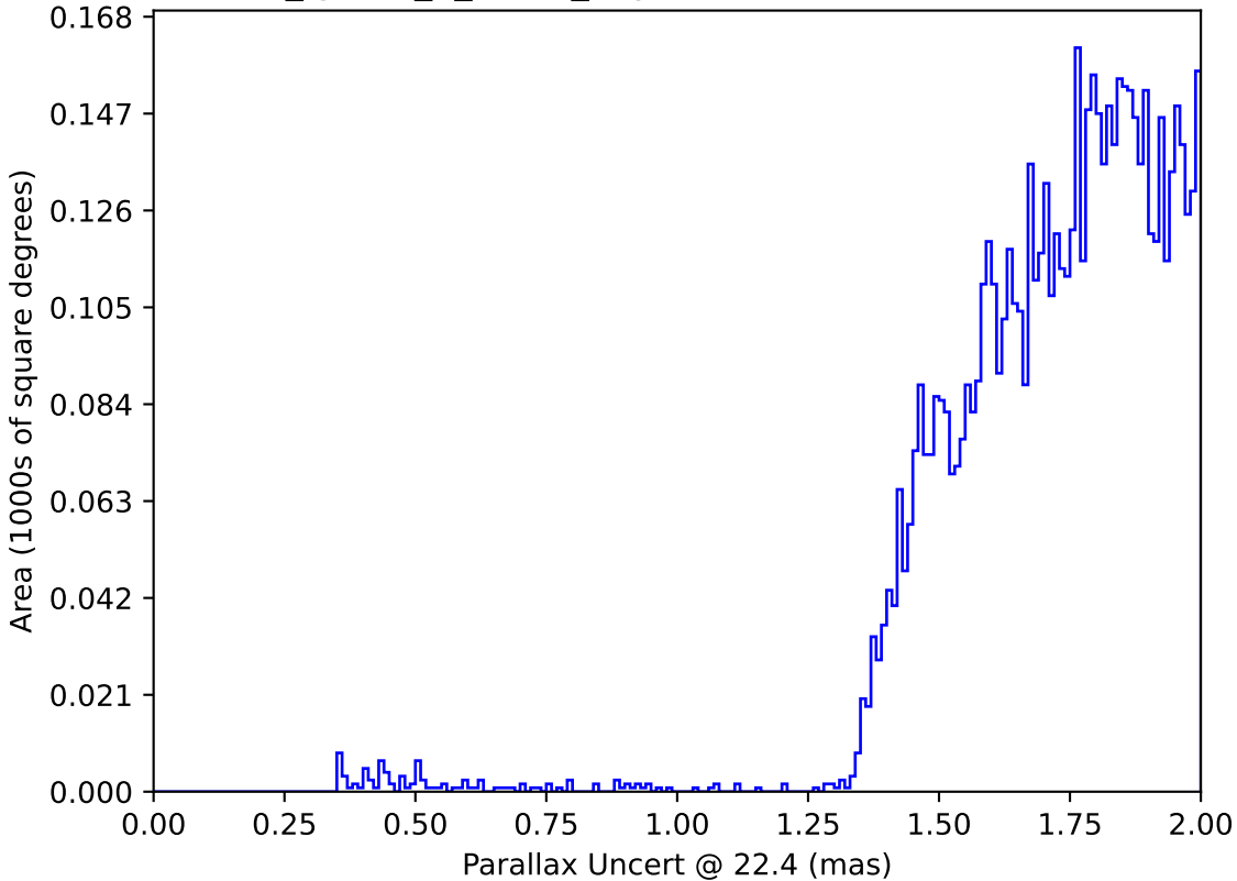
too_ignore_5_4v3.4_10yrs : Parallax Uncert @ 22.4
