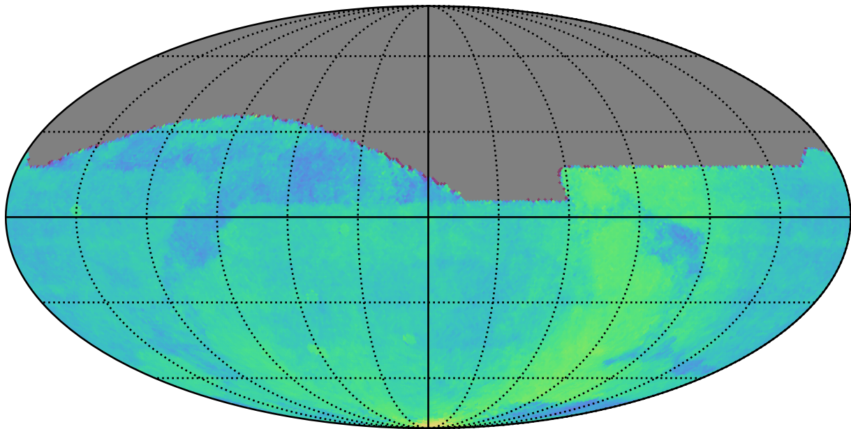
too_ignore_5_4v3.4_10yrs : Parallax Coverage @ 22.4
