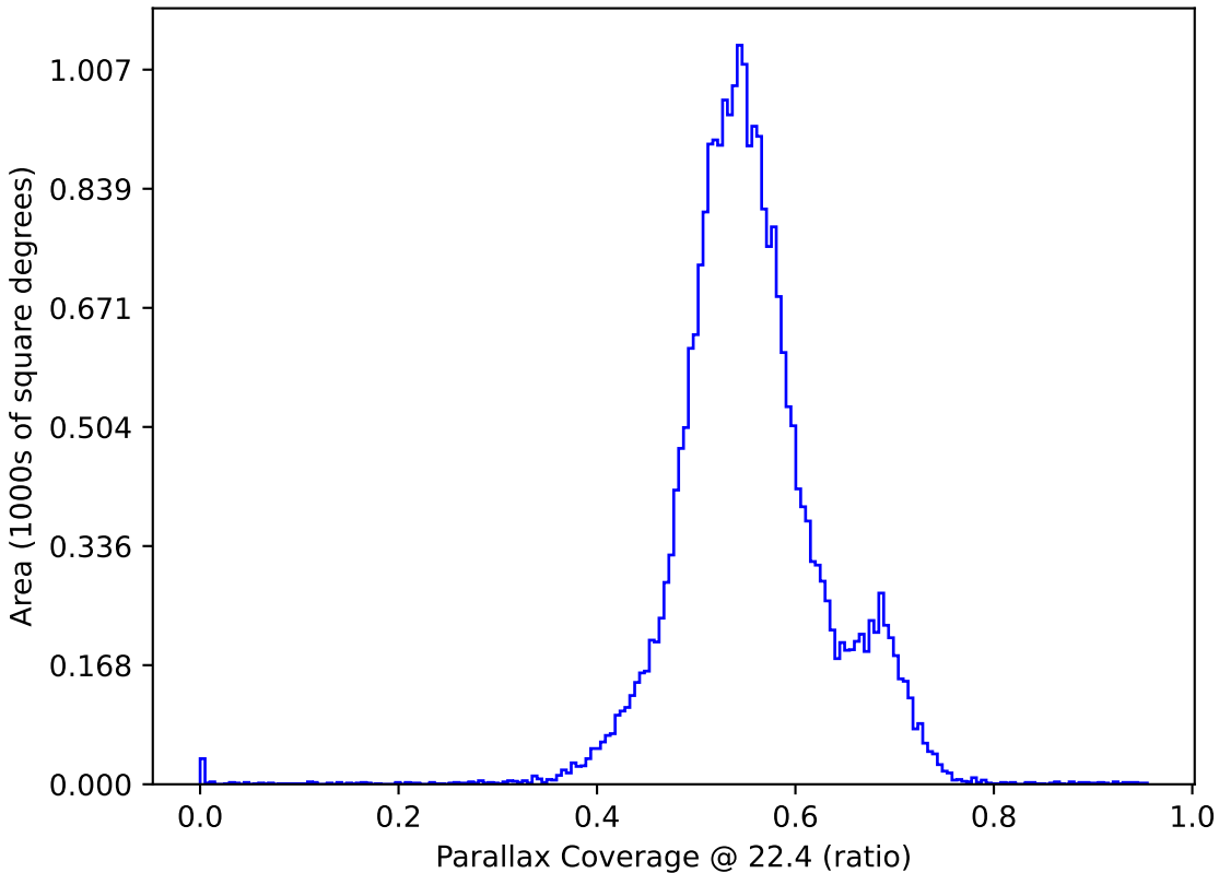
too_ignore_5_4v3.4_10yrs : Parallax Coverage @ 22.4
