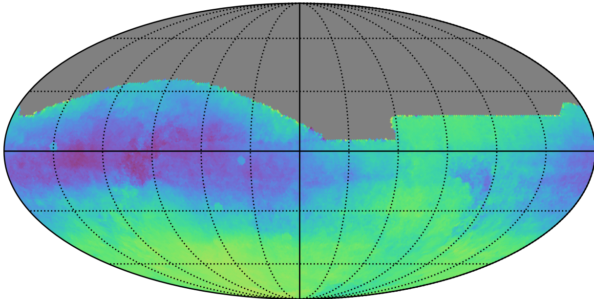
too_ignore_5_4v3.4_10yrs : Parallax-DCR degeneracy @ 24.0
