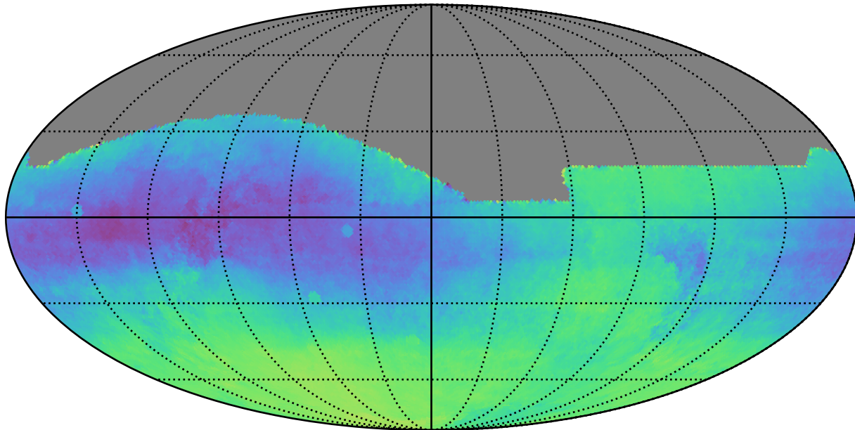
too_ignore_5_4v3.4_10yrs : Parallax-DCR degeneracy @ 22.4
