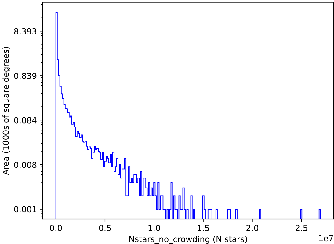
too_ignore_5_4v3.4_10yrs z: Nstars_no_crowding
