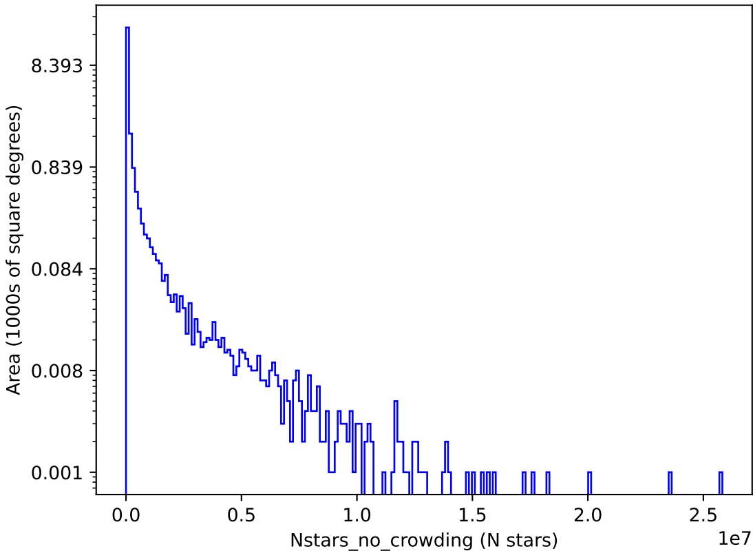
too_ignore_5_4v3.4_10yrs y: Nstars_no_crowding
