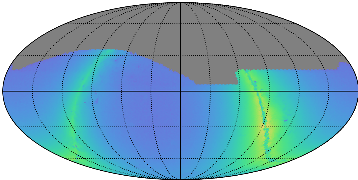
too_ignore_5_4v3.4_10yrs r: Nstars_no_crowding
