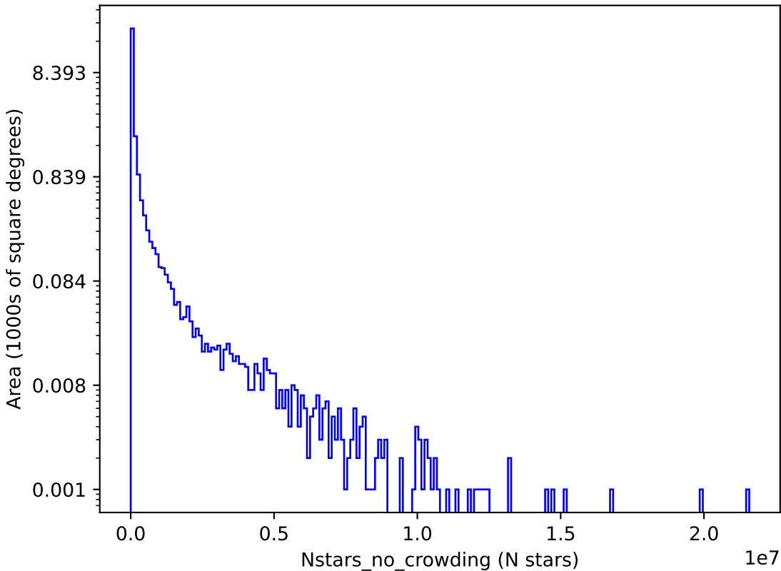
too_ignore_5_4v3.4_10yrs r: Nstars_no_crowding
