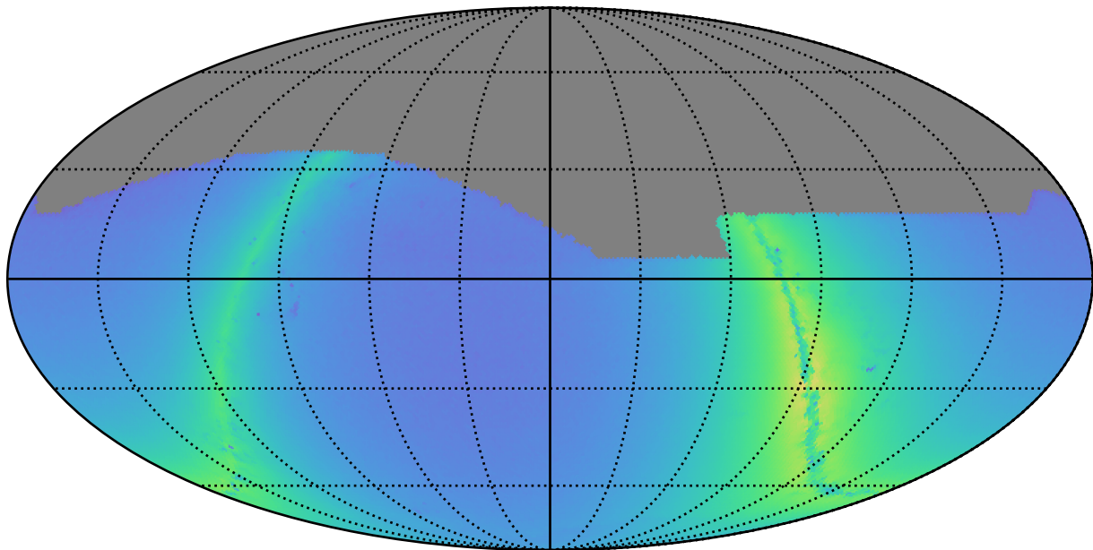
too_ignore_5_4v3.4_10yrs i: Nstars_no_crowding
