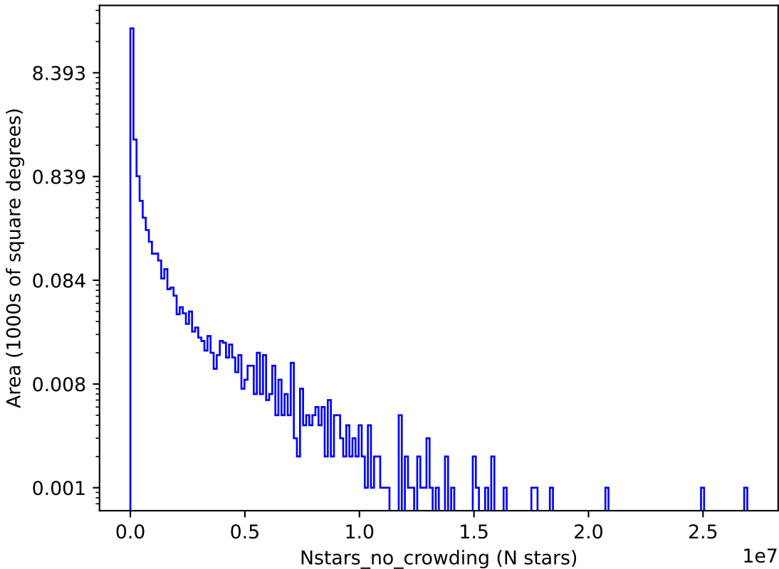
too_ignore_5_4v3.4_10yrs i: Nstars_no_crowding
