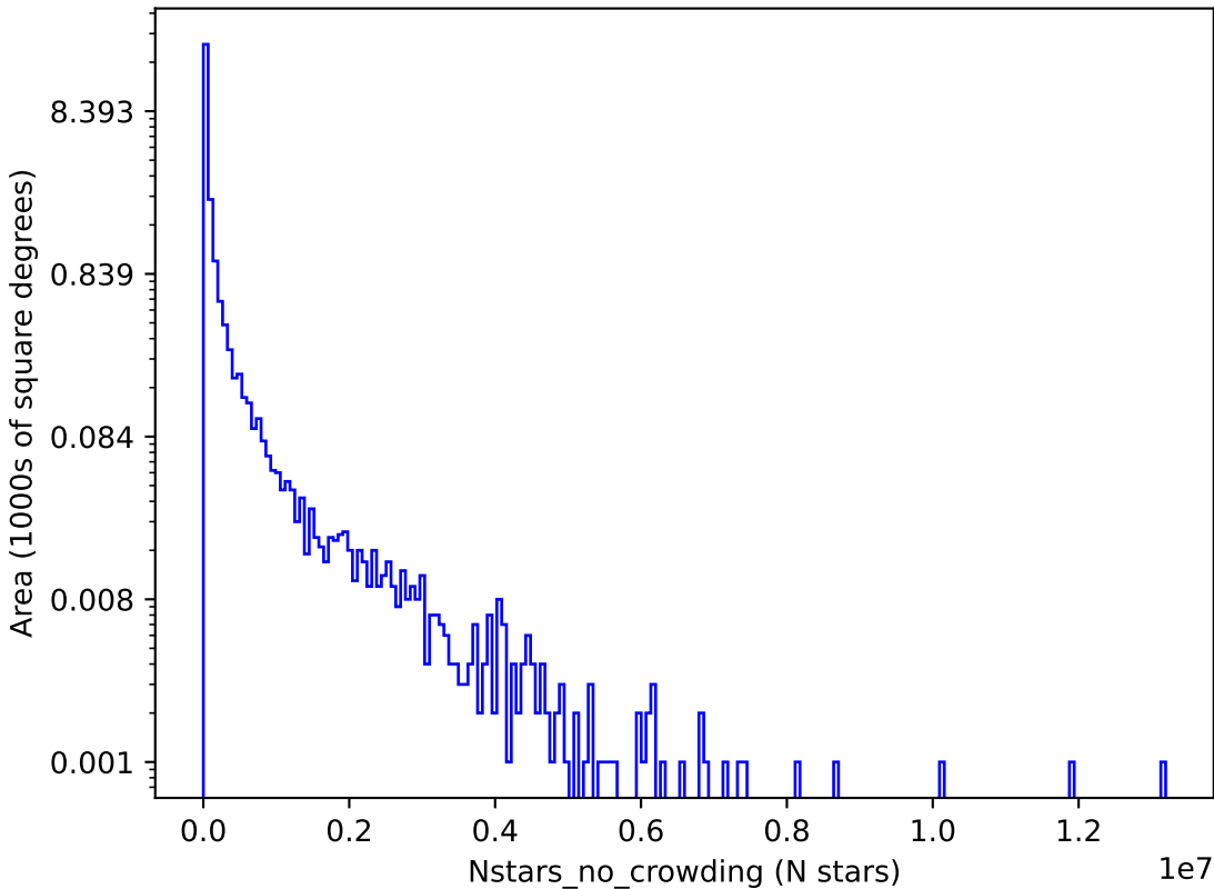
too_ignore_5_4v3.4_10yrs g: Nstars_no_crowding
