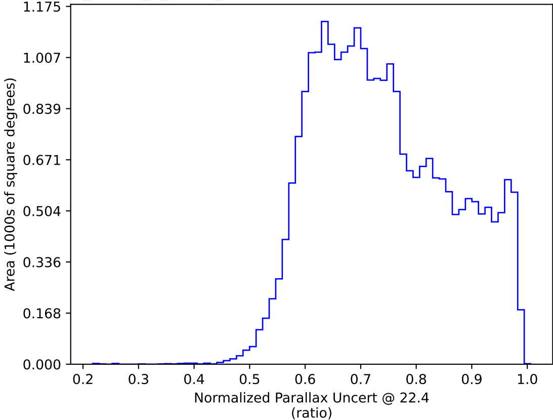
too_ignore_5_4v3.4_10yrs : Normalized Parallax Uncert @ 22.4
