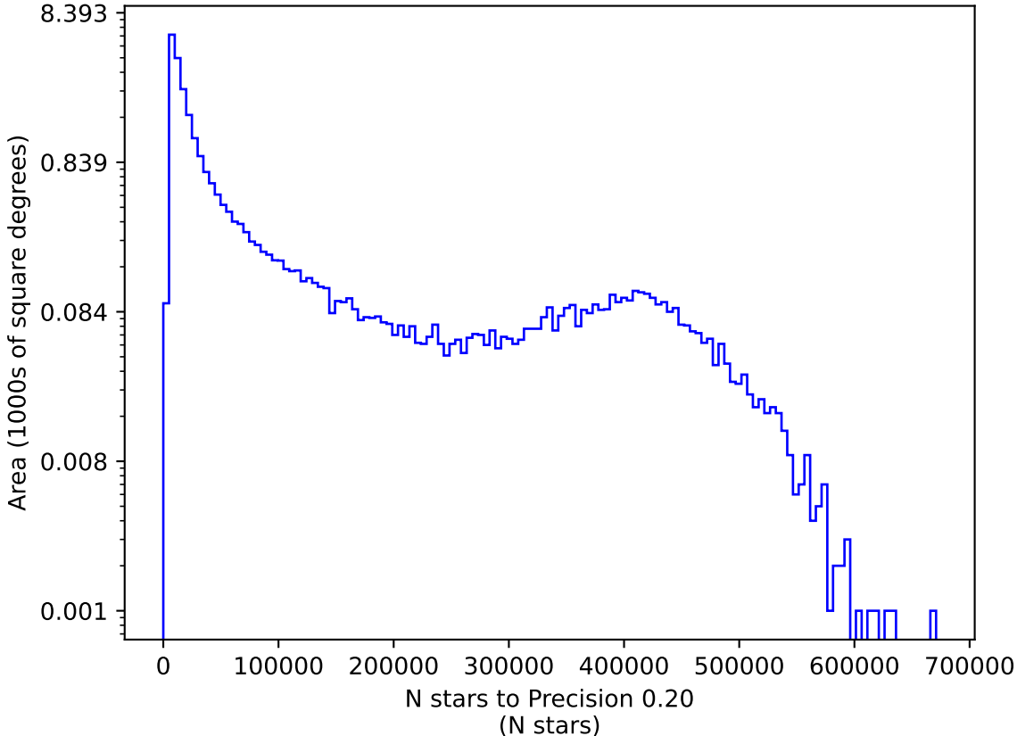
too_ignore_5_4v3.4_10yrs z: N stars to Precision 0.20
