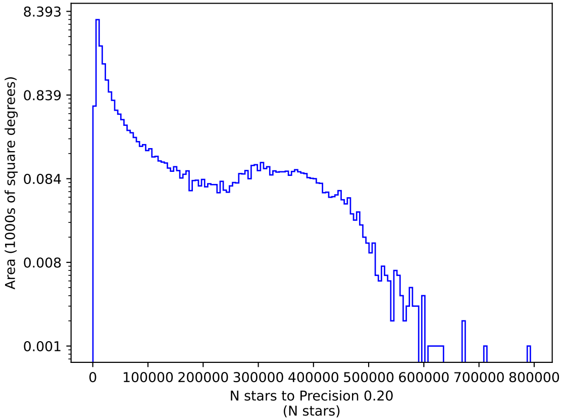
too_ignore_5_4v3.4_10yrs y: N stars to Precision 0.20
