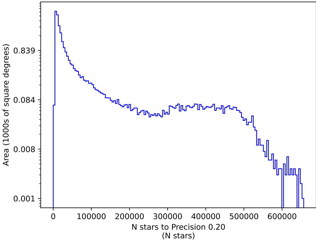
too_ignore_5_4v3.4_10yrs r: N stars to Precision 0.20
