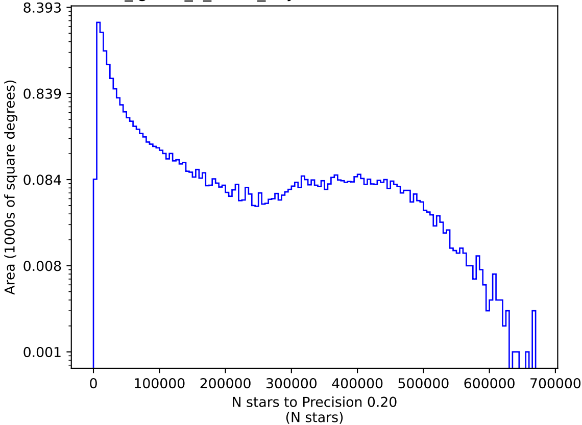
too_ignore_5_4v3.4_10yrs i: N stars to Precision 0.20
