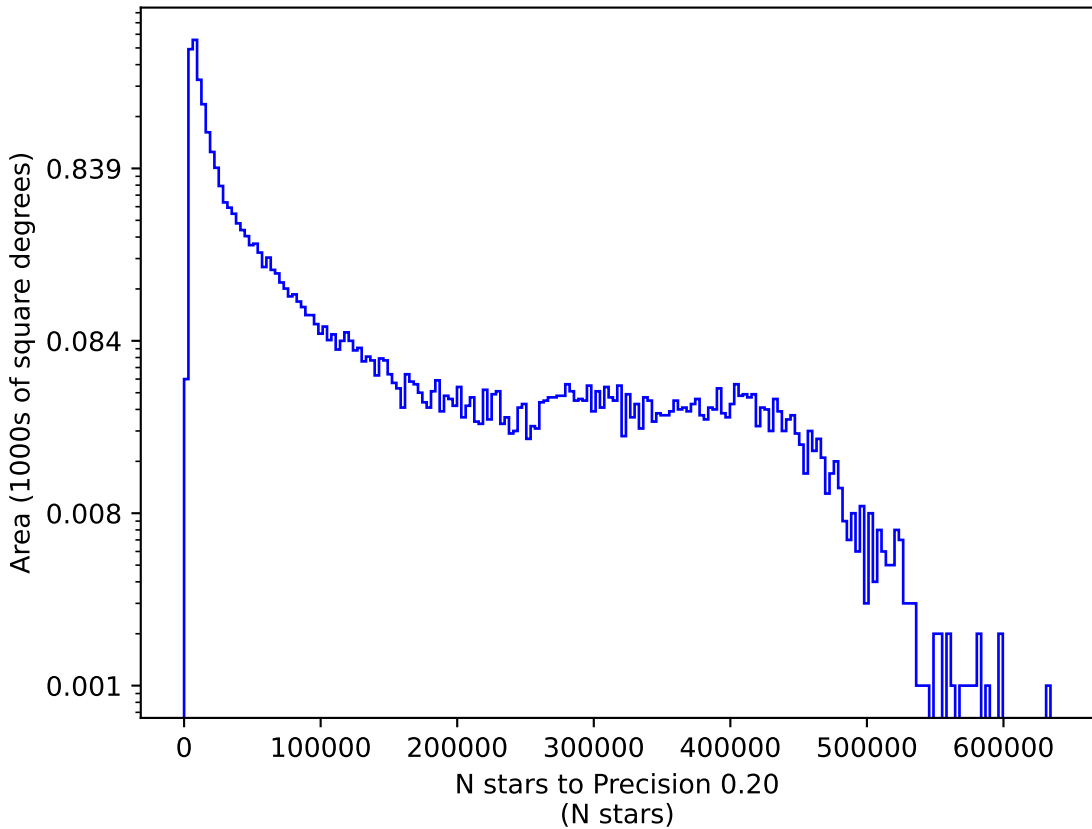
too_ignore_5_4v3.4_10yrs g: N stars to Precision 0.20
