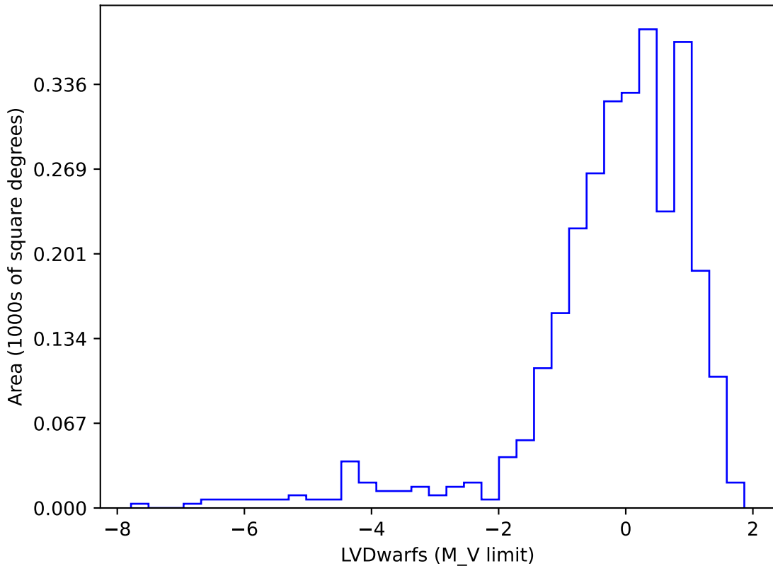
too_ignore_5_4v3.4_10yrs gi SCP: LVDwarfs
