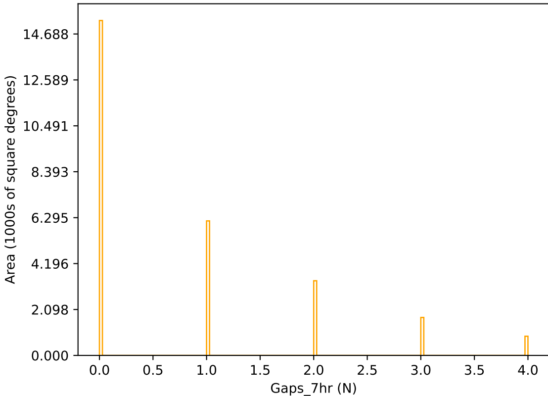
too_ignore_5_4v3.4_10yrs r band: Gaps_7hr
