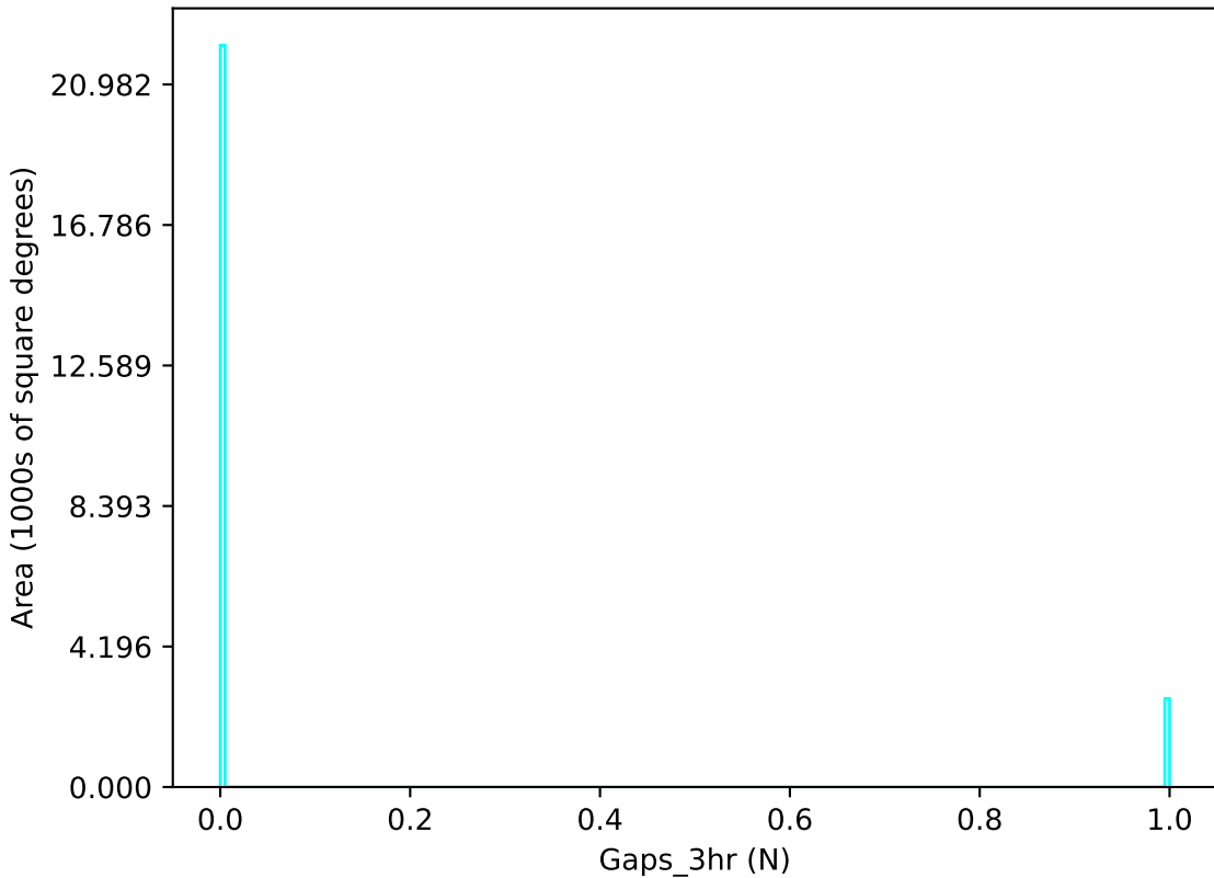
too_ignore_5_4v3.4_10yrs u band: Gaps_3hr
